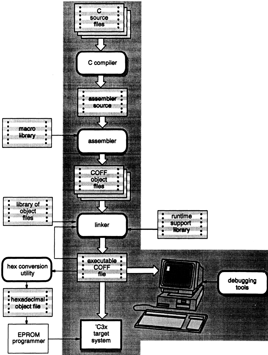
Figure 1-3. 'C3x Software Development Flow
