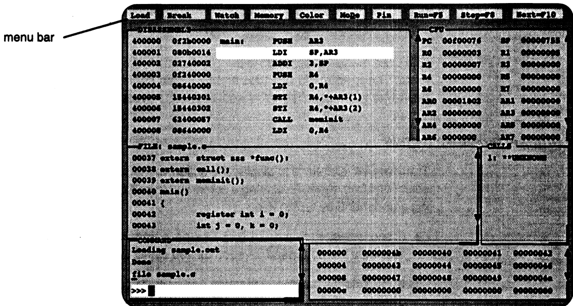
Figure 4-2. The Menu Bar in the Basic Debugger Display
