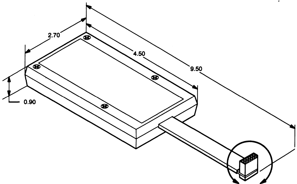
Figure A-4. Pod/Connector Dimensions
